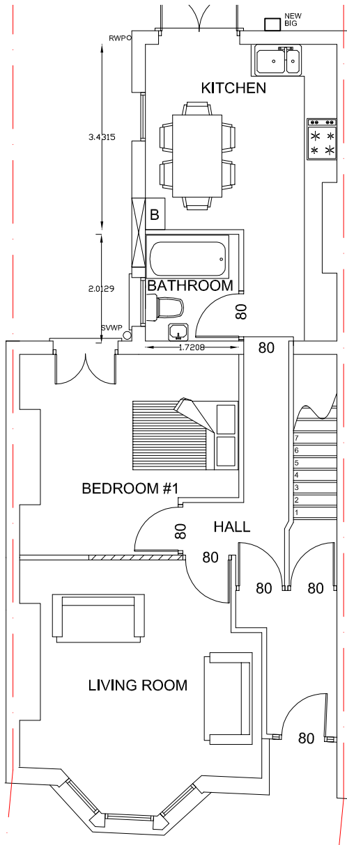
PROPOSED GROUND FLOOR FLAT PLAN SCALE: N/A
